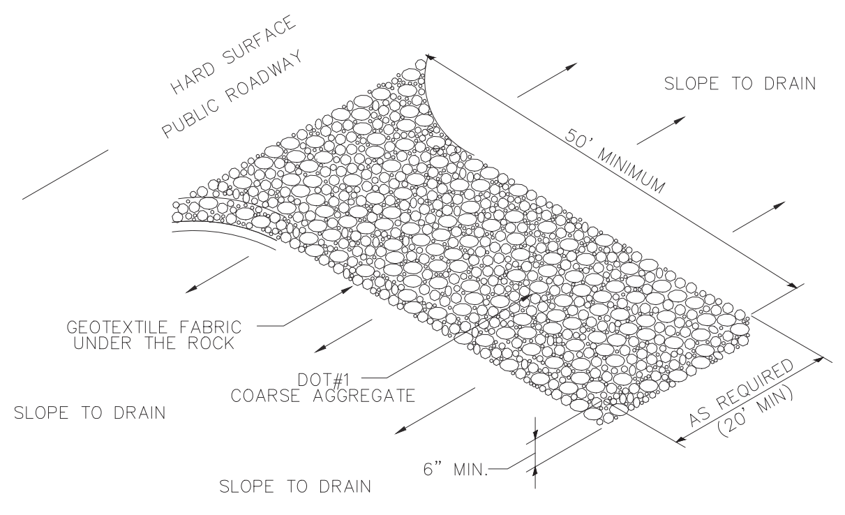
TEMPORARY CONSTRUCTION ENTRANCE AND EXIT SCALE: N.T.S. UPDATED: 4/5/05
