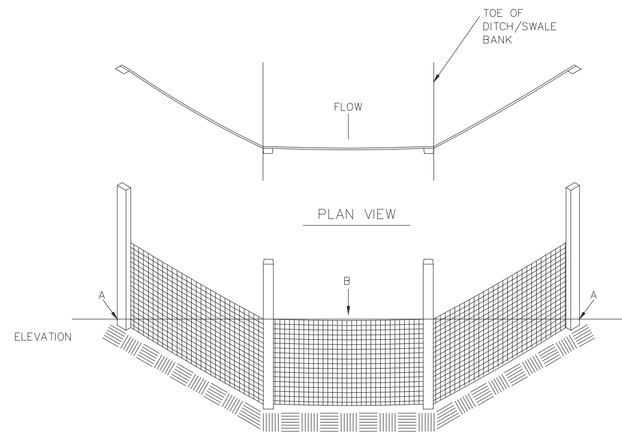
POINTS A SHOULD BE HIGHER THAN POINT B SILT FENCE DITCH/SWALE PROTECTION
