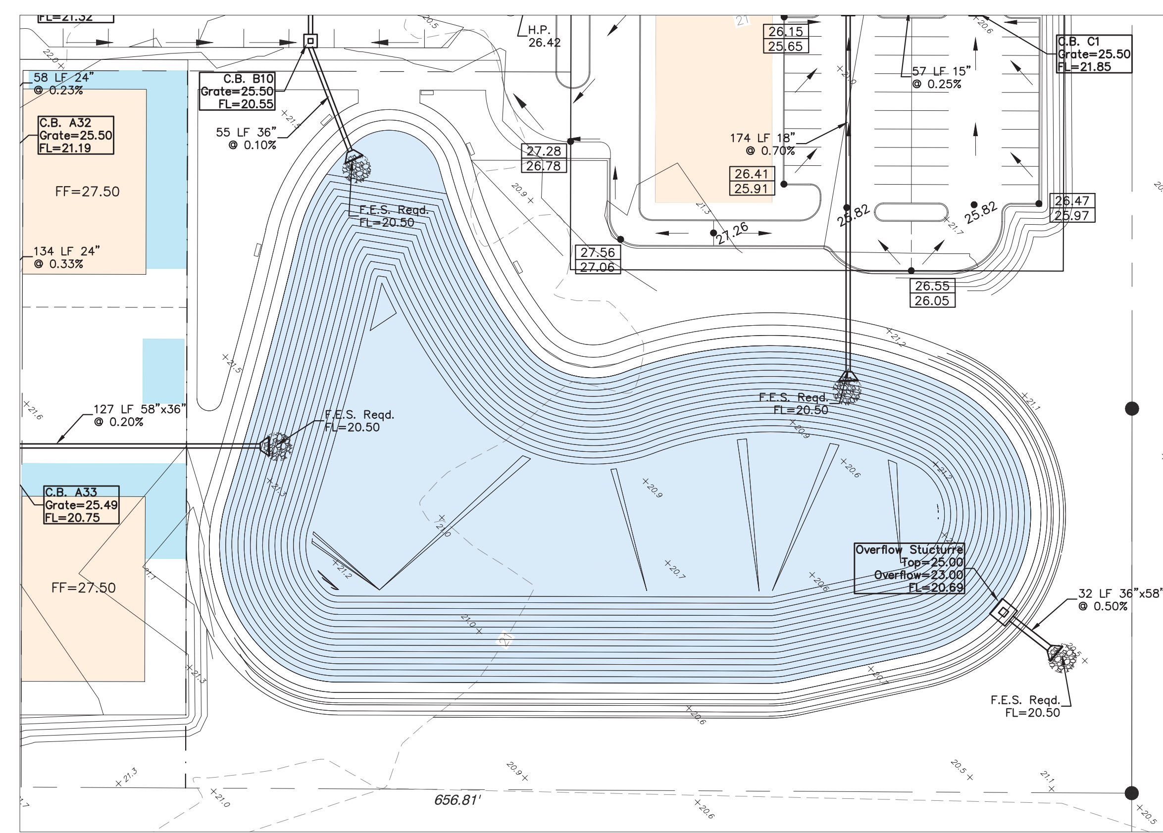
Site Plan
