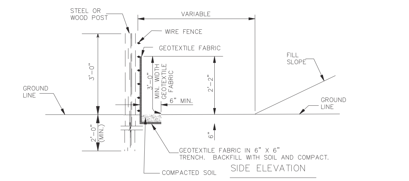
TEMPORARY SILT FENCING
