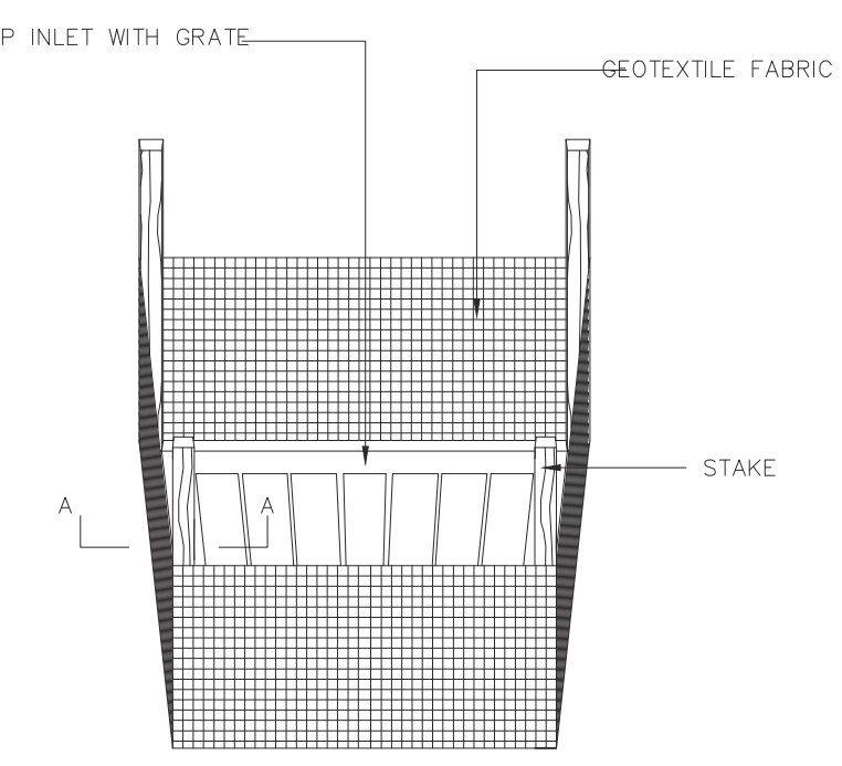
SILT FENCE INLET PROTECTION
